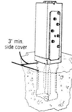
Typical CBSQ-SDS2 Installation
